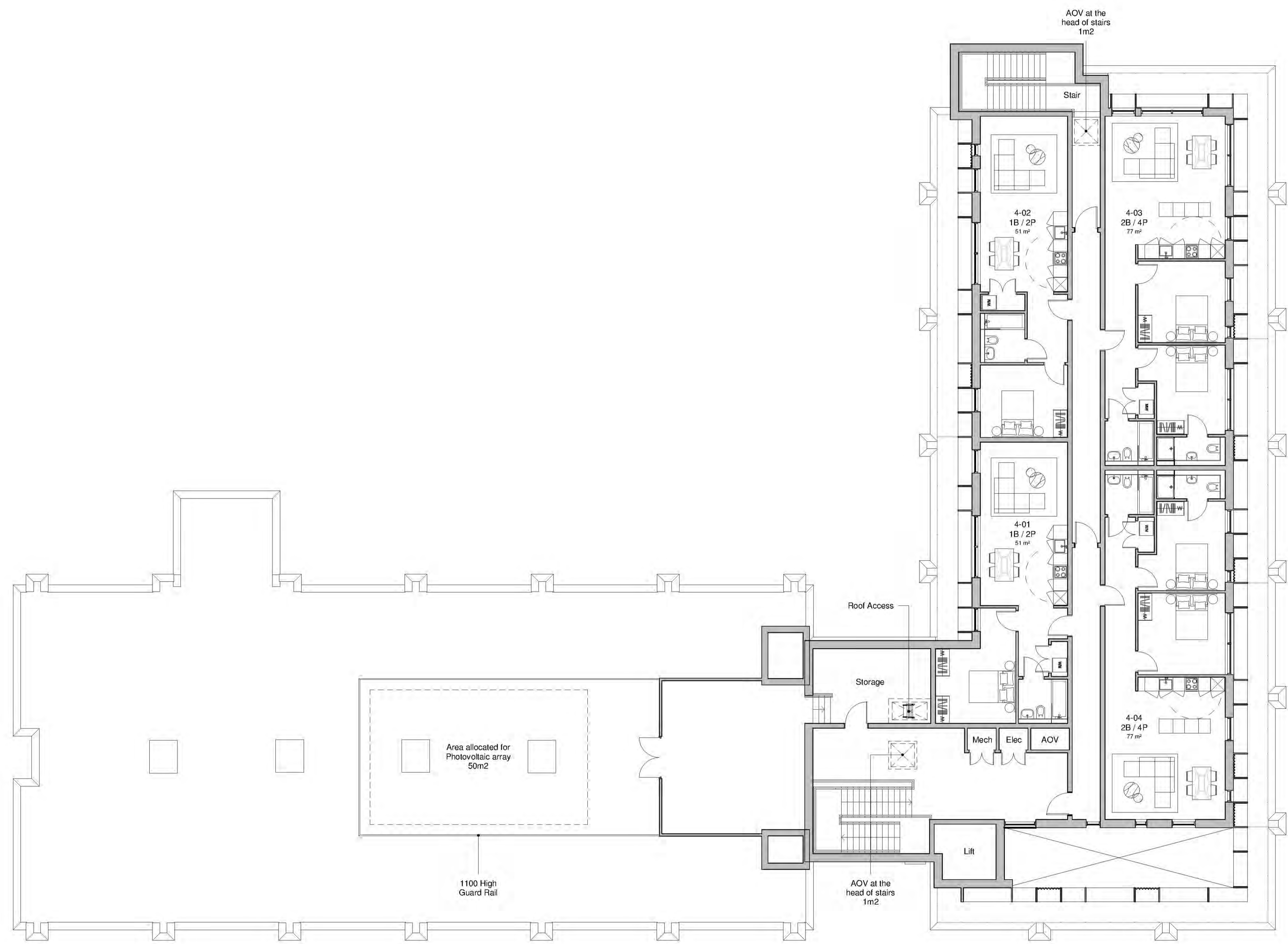
04 Proposed Fourth Floor NB.1 1:100
